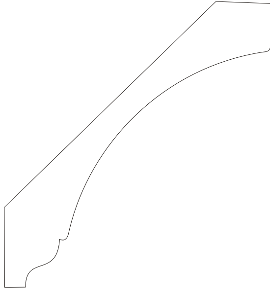
MM016-S 3/4 x 4-1/16 crown Copyright Flex Trim, Inc. 2005
