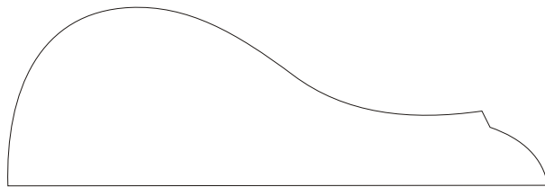
FRANKLIN-S 1-1/16 x 3-1/4 casing Copyright Flex Trim, Inc. 2006
